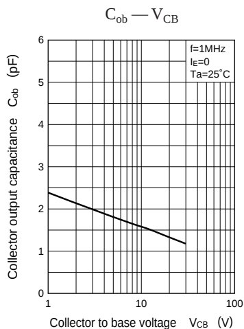
Characteristics charts of UN521T
