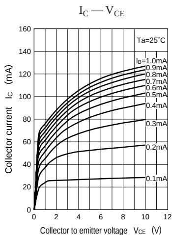
Characteristics charts of UN521T
