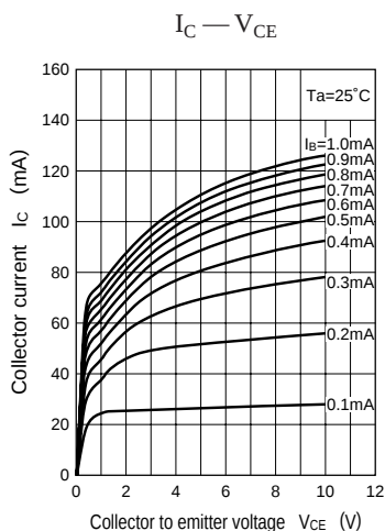
Characteristics charts of UN521N
